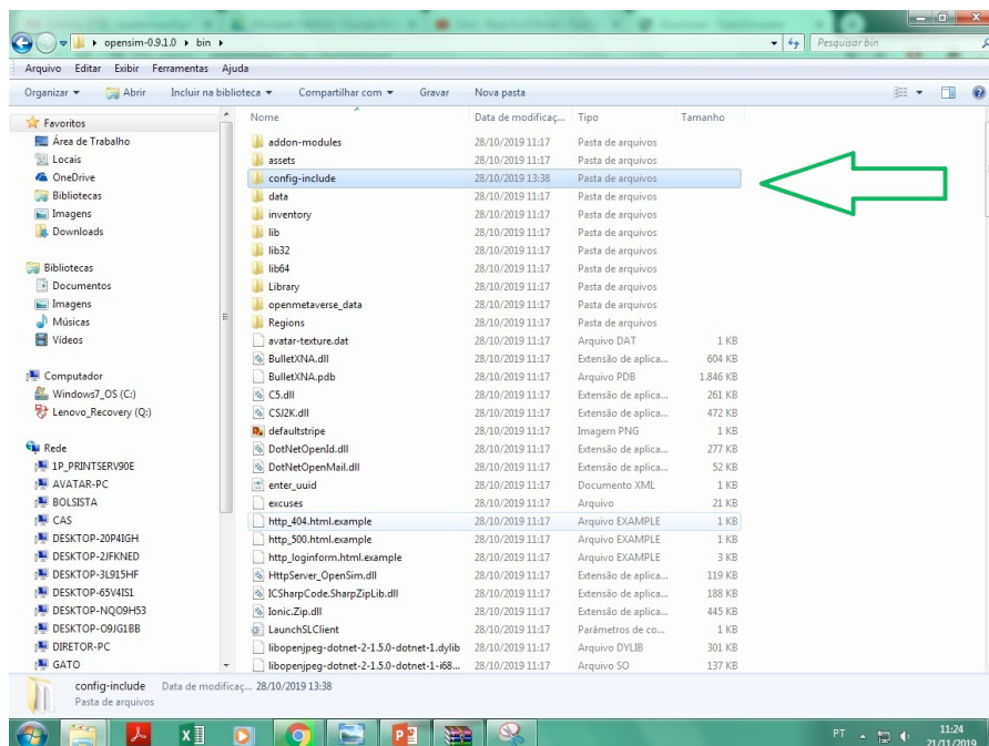
Figura 2.30 - Pasta “config-include”.
